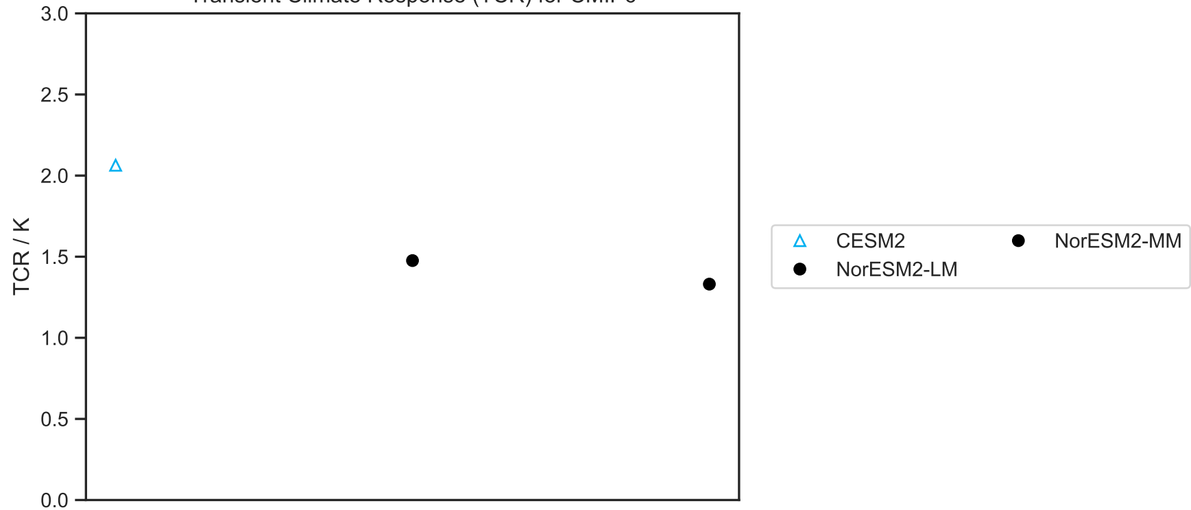
Transient Climate Response (TCR) for CMIP6
