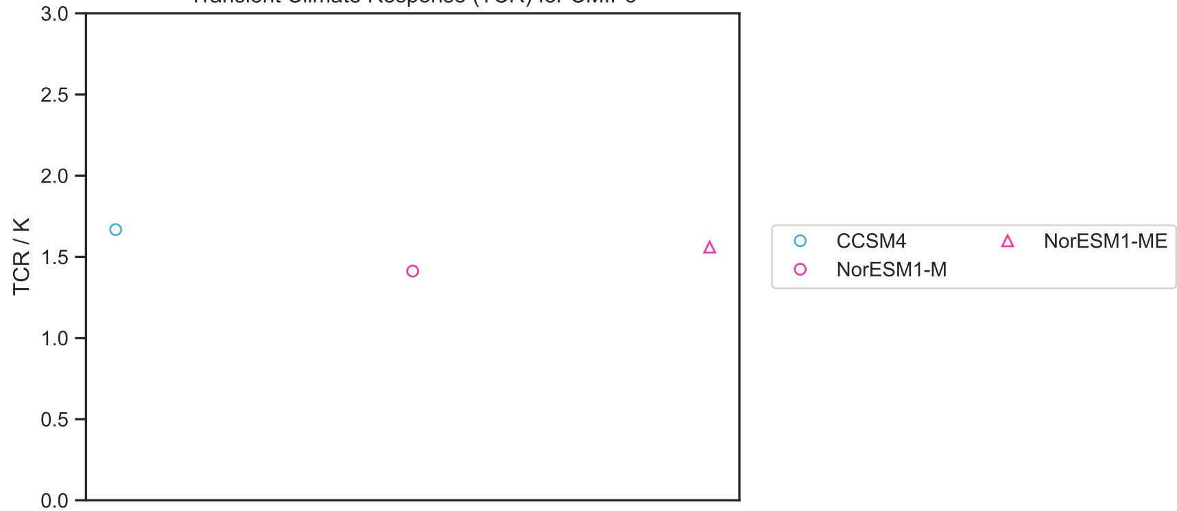
Transient Climate Response (TCR) for CMIP5
