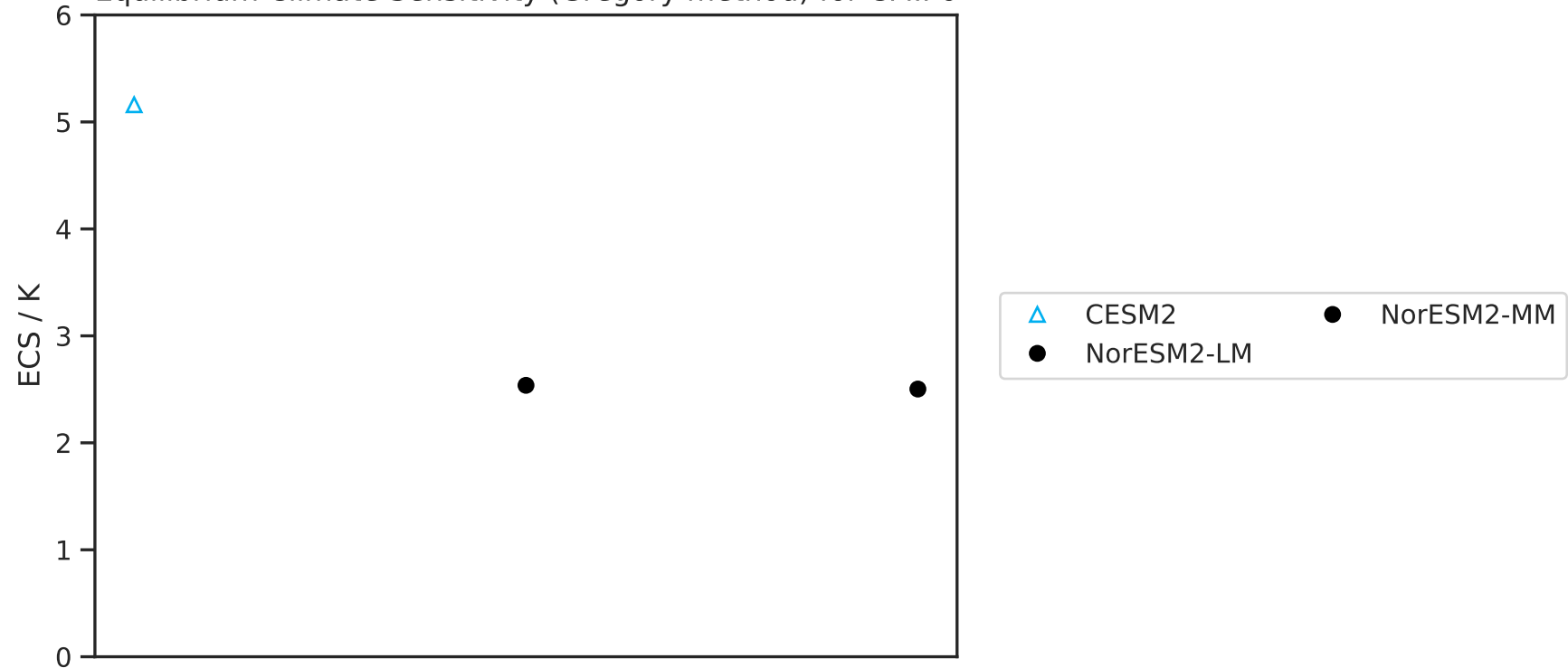
Equilibrium Climate Sensitivity (Gregory method) for CMIP6
