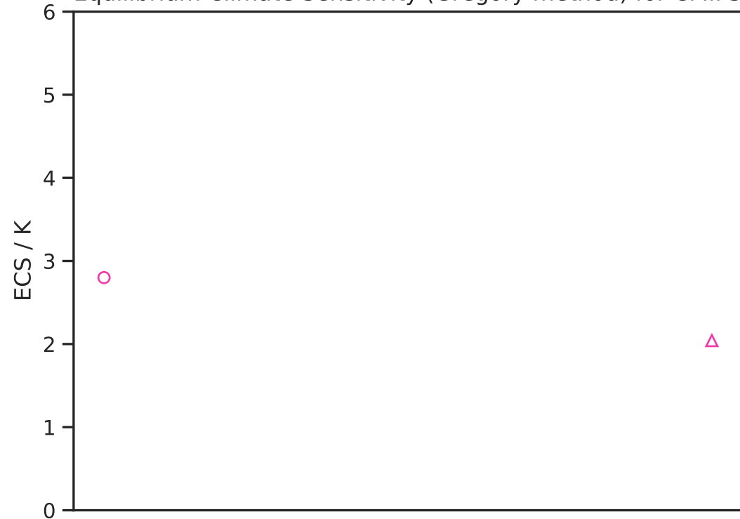
Equilibrium Climate Sensitivity (Gregory method) for CMIP5
